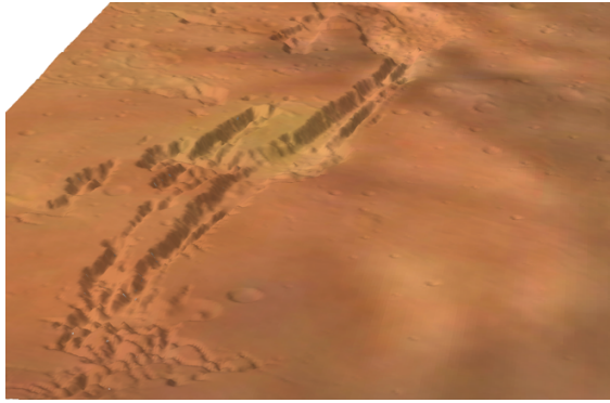
Figure 4: Dust accumulation in Sinai Planum on 1 August 2018.
